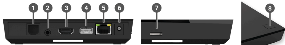
Figure 1 : Raccordements
